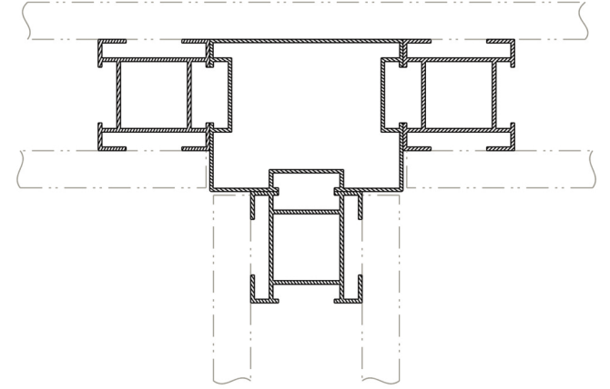
POTEAU 3 DEPARTS
